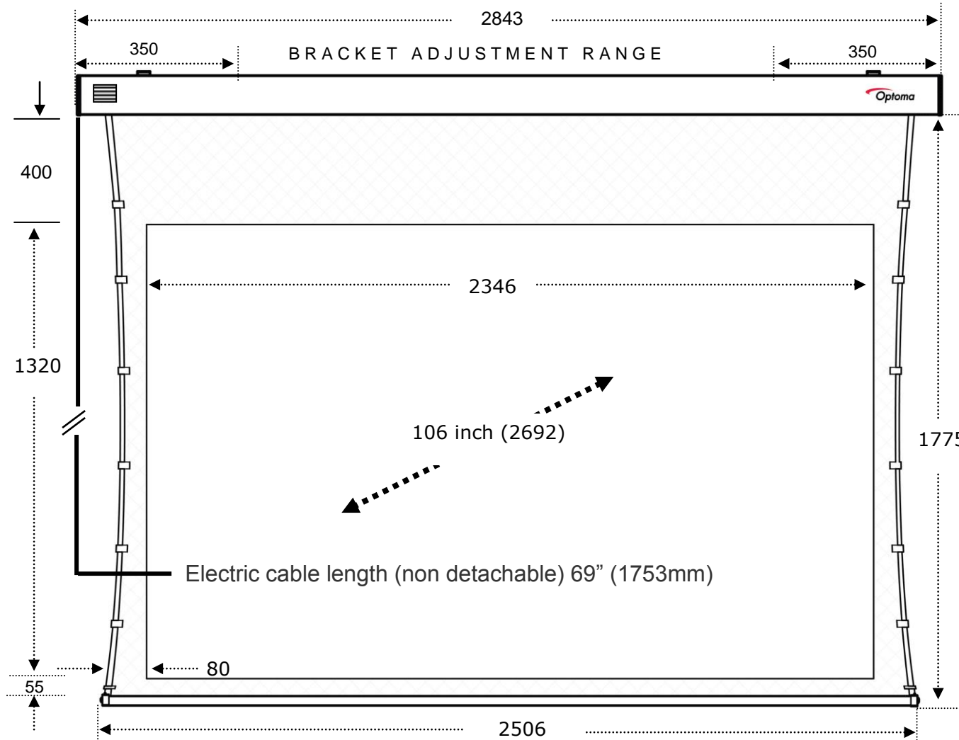
Optoma 16:9 DE-9106ETT ELECTRIC SCREEN Measurements in Milimetres
