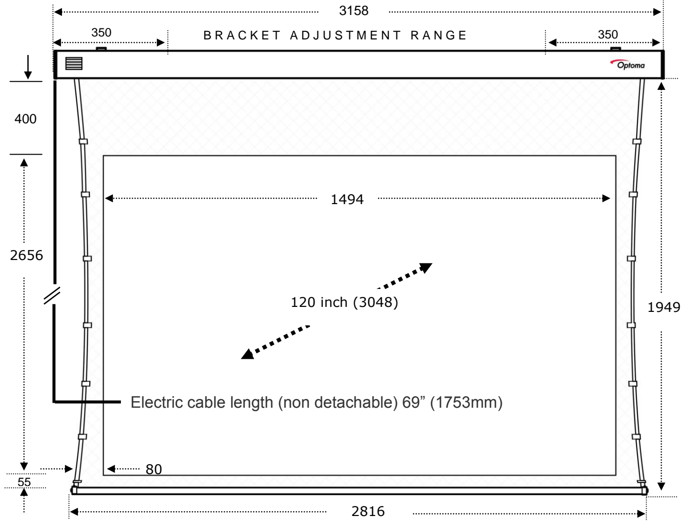
Optoma 16:9 DE-9120ETT ELECTRIC SCREEN Measurements in Millimetres
